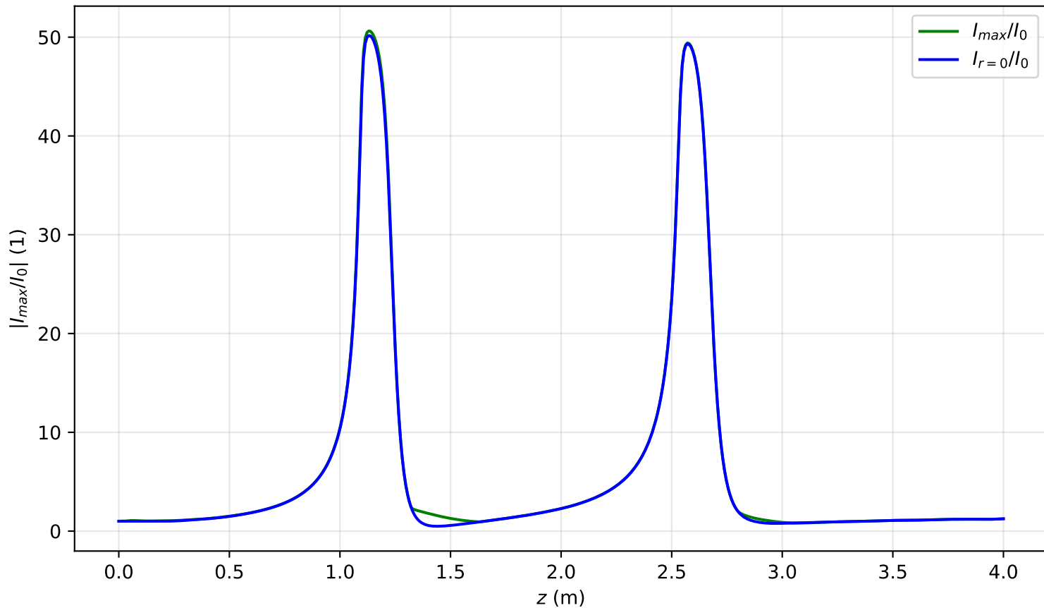
I_{max}(x=0, y=0, z)/I_0 , \text{Pin}=2.1\text{Pcr} , noisy input, artificial time
